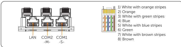
Figure 6-22 Communication ports
