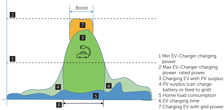
Figure 9-13 Timer Boost
